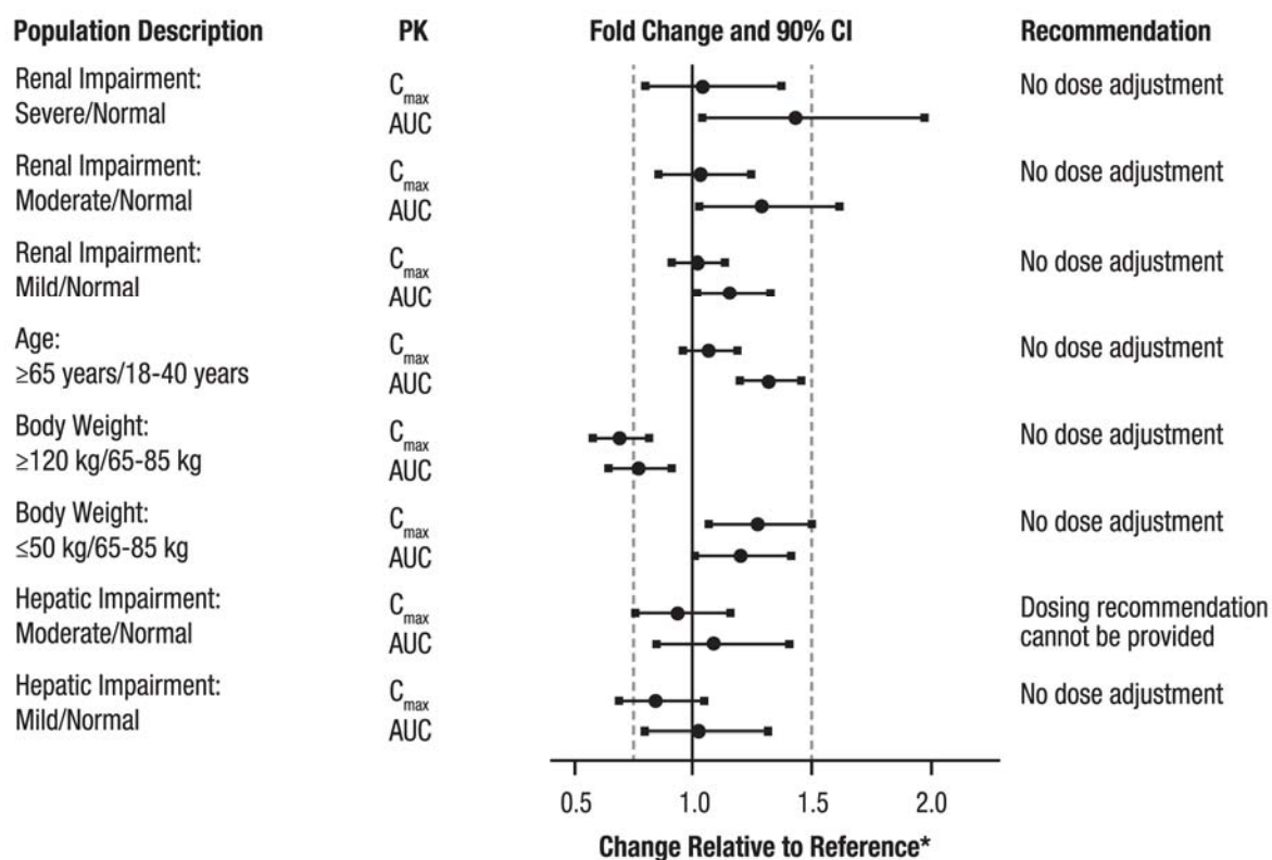
Figure 3: Effect of Specific Populations on the Pharmacokinetics of Apixaban
